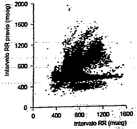
Intervalos RR
