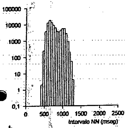
Histograma NN
