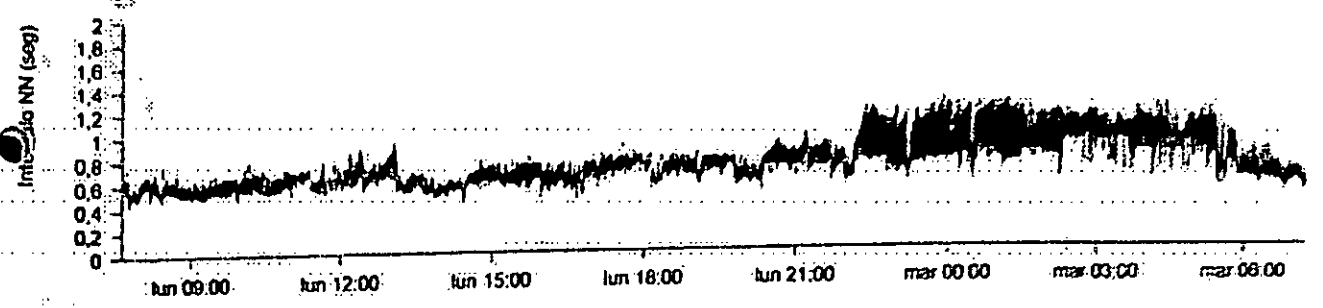
Intervalos RR
